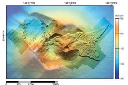
Topography of a submarine volcano revealed using an AUV
